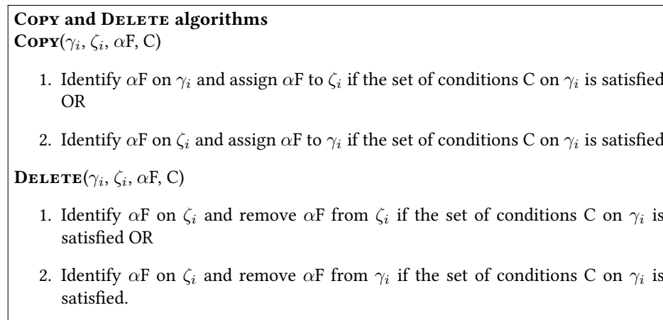
Figure 1.2: COPY &amp; DELETE algorithms
